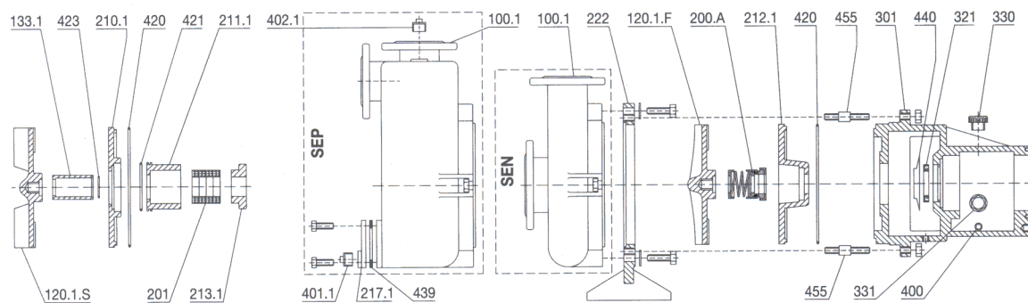
Gland Packing
